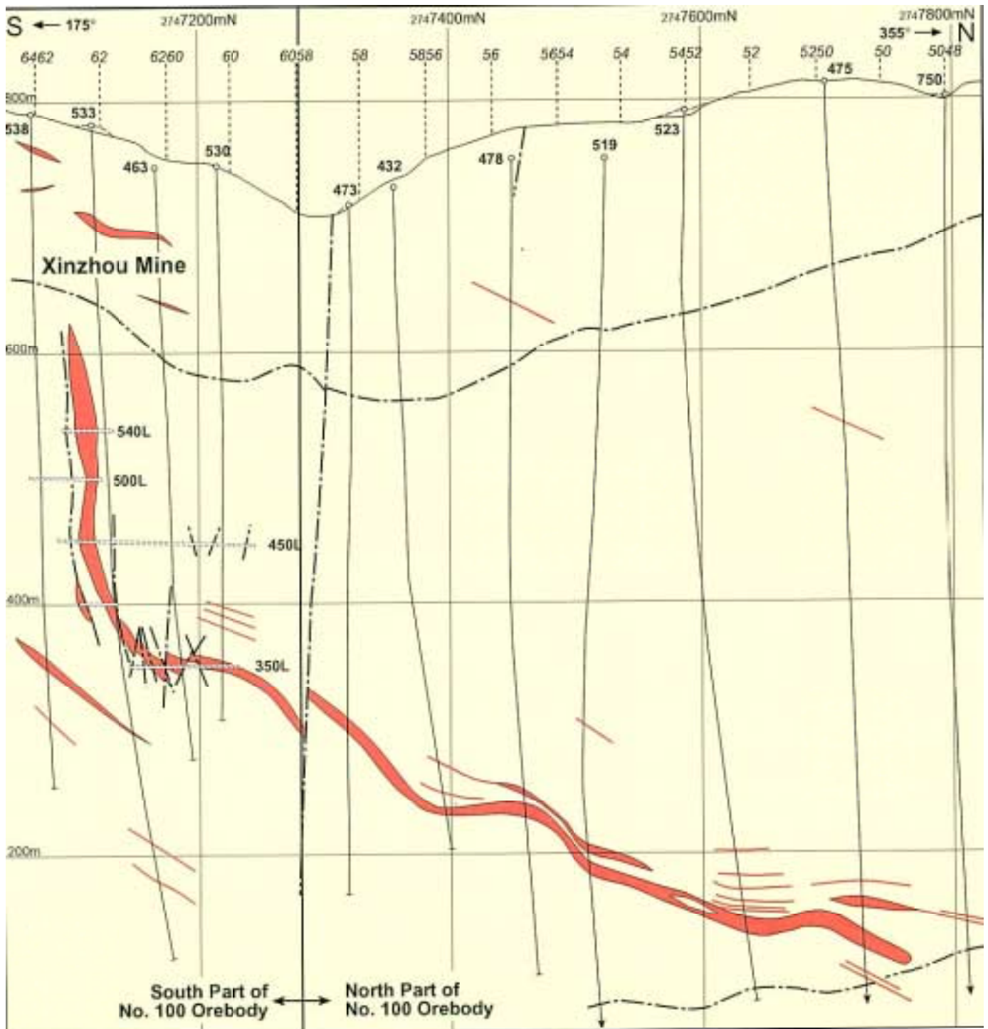
Figure 7 Biogan International, Inc. No. 100 Orebody Gaofeng Mine Longitudinal Section (after Anon, 1994)
